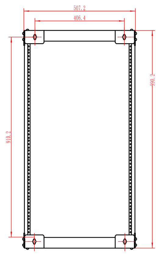
Back View
