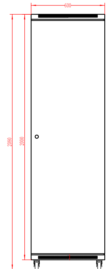
REAR DOOR
