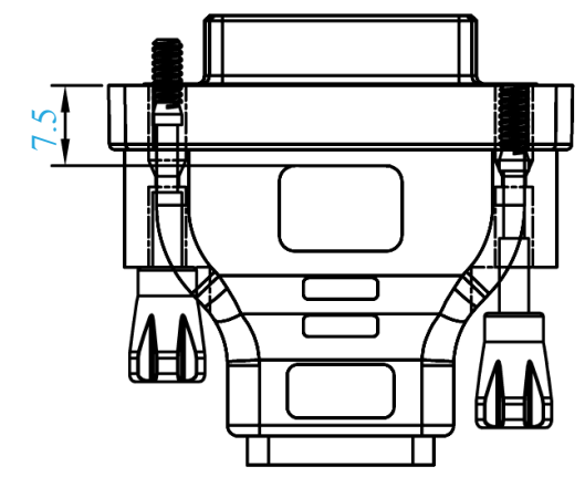
DVI-D 24+1 Male
