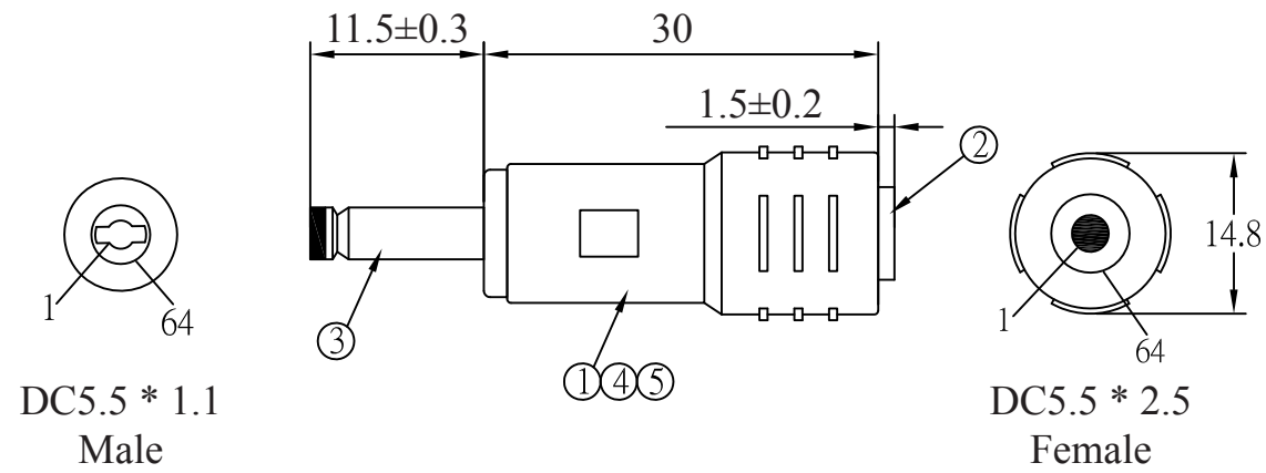
Black Adapter TOL: ± 0.5mm
